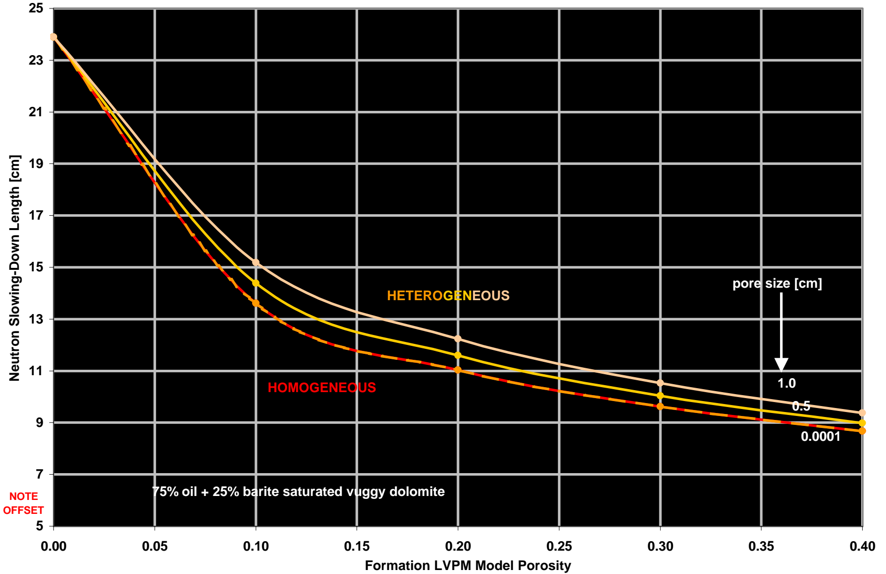
Neutron Slowing-Down Length vs Formation LVPM Model Porosity
